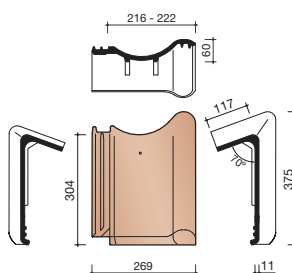
8500 CHAPERONPAN
